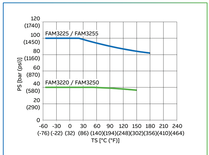
Figure 3: PS: pressure, TS: temperature
