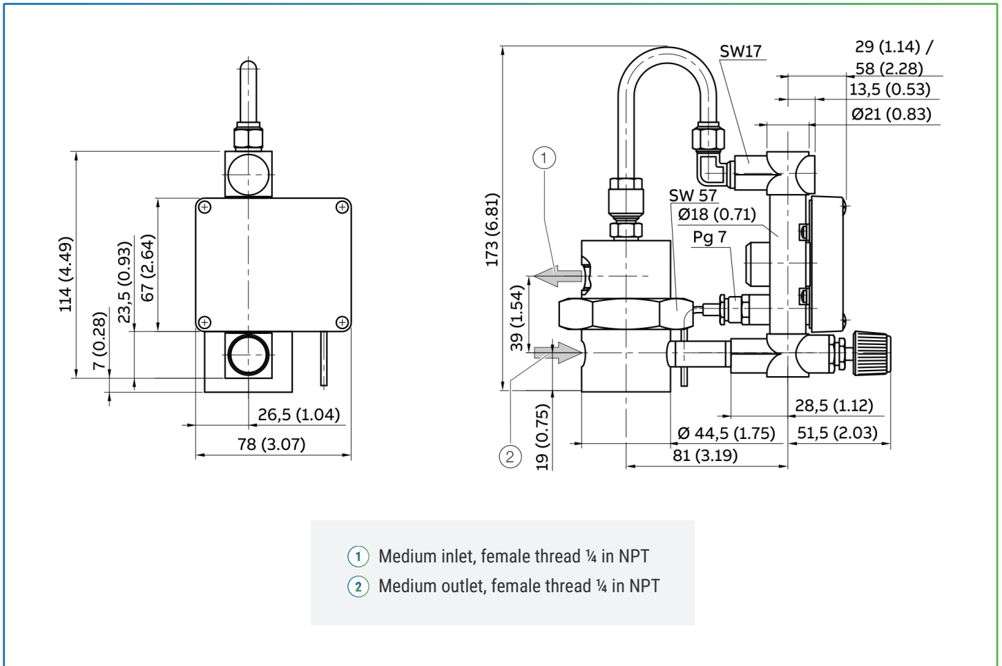
Figure 10: Dimensions in mm (in), projection in accordance with ISO method E
