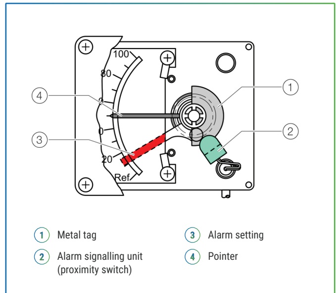
Figure 4: Single alarm (example)
