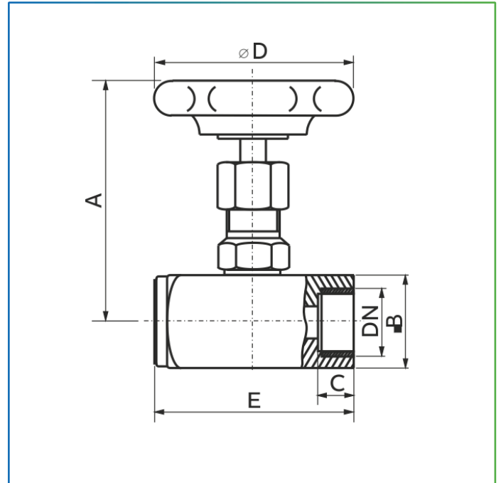
Figure 12: Stainless steel needle valve
