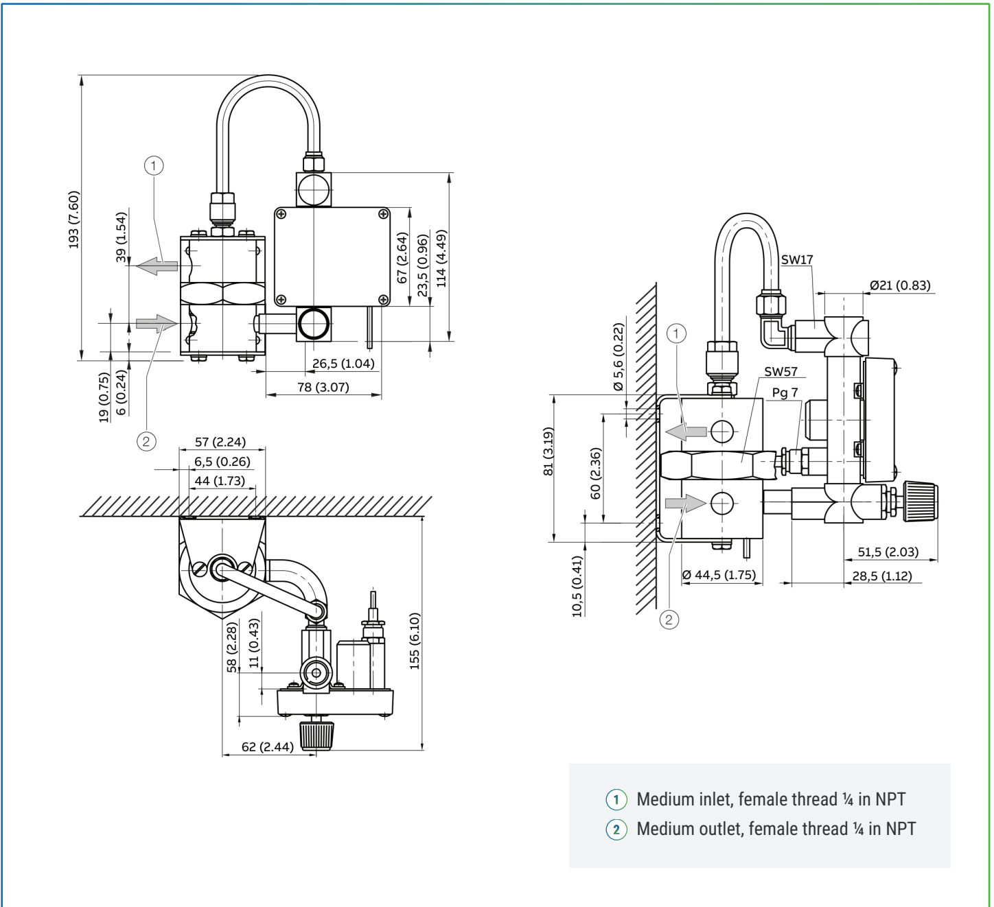
Figure 9: Dimensions in mm (in), projection in accordance with ISO method E
